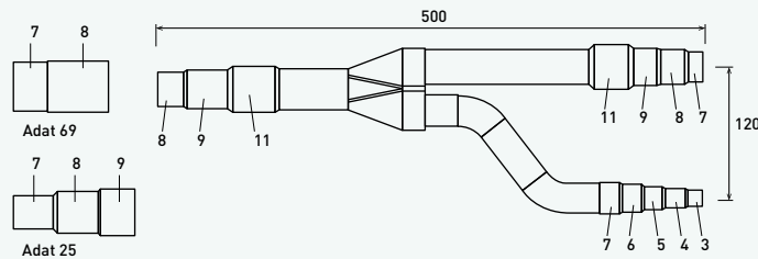
Gas piping
