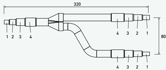
Liquid piping
